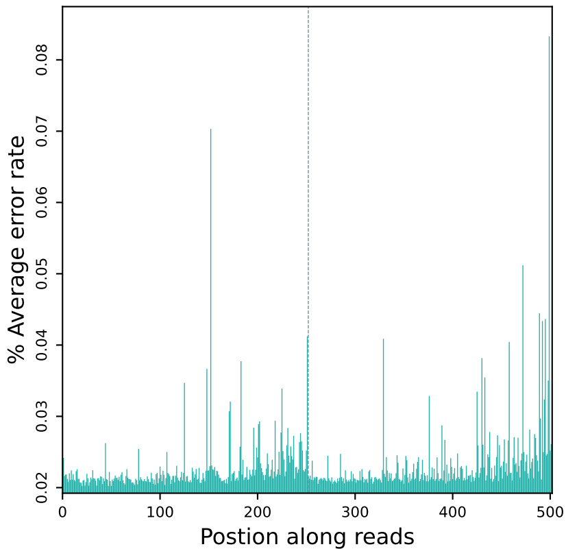
Error rate distribution along reads (R10607)
